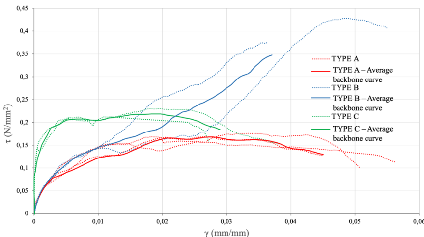
Figure 16. Stress-strain curves of the three types of specimens under shear and compression loads.
