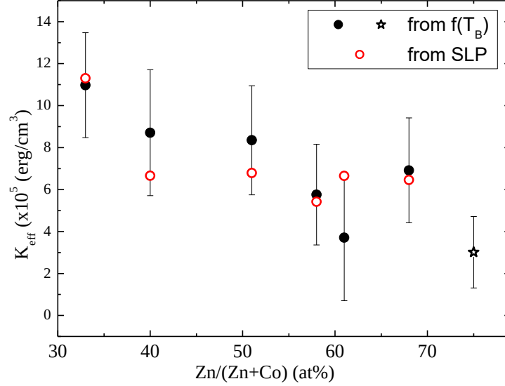
Figure 4. Magnetic anisotropy estimated from \langle T_B \rangle , V_{mag} , and \tau_0 = 2(1) \cdot 10^{-11} s experimental parameters, (solid black dots) and calculated from the SLP measurements (open red dot) as function of Zn/(Zn+Co) atomic shell ratio. The magnetic anisotropy of the core, estimated from \langle T_B \rangle , is also presented with empty star.
