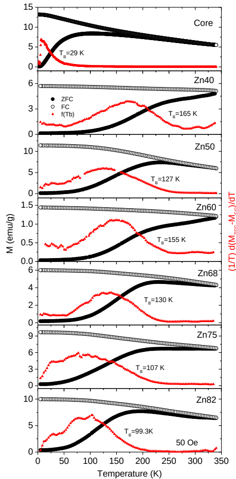
Figure 3. Temperature dependence of the M_{ZFC}(T) and M_{FC}(T) curves of the core and \text{Fe}_3\text{O}_4/\text{Zn}_x\text{Co}_{1-x}\text{Fe}_2\text{O}_4 NPs with 0.2 wt% in Epoxy resin and measured under applied field of 50 Oe. The red triangles is the distributions of blocked temperature f(T_B) for each sample calculated from Equation 4.
