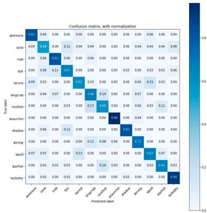
Figure A10. Confusion matrix for the classification results (accuracy) obtained by CNN-3.
