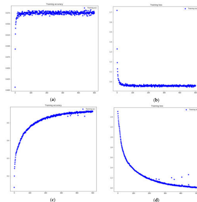
Figure 7. Training accuracy and loss plots of the DNNs with different structures. The X axis of all of plots shows the number of epochs, while the Y axis show the loss or accuracy value that reached the trained model. Training accuracy and loss plots of DNN-1: (a) Accuracy values obtained in every epoch at training time and (b) loss values obtained in every epoch at training time. Training accuracy and loss plots of DNN-4: (c) Accuracy values obtained in each epoch at training time and (d) loss values obtained in each epoch at training time.
