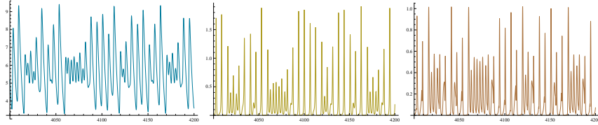
Figure 7: The time series of the functions x , y , z on the attractor \mathcal{A}_1 for the choice of the parameters as in section 4.2.
