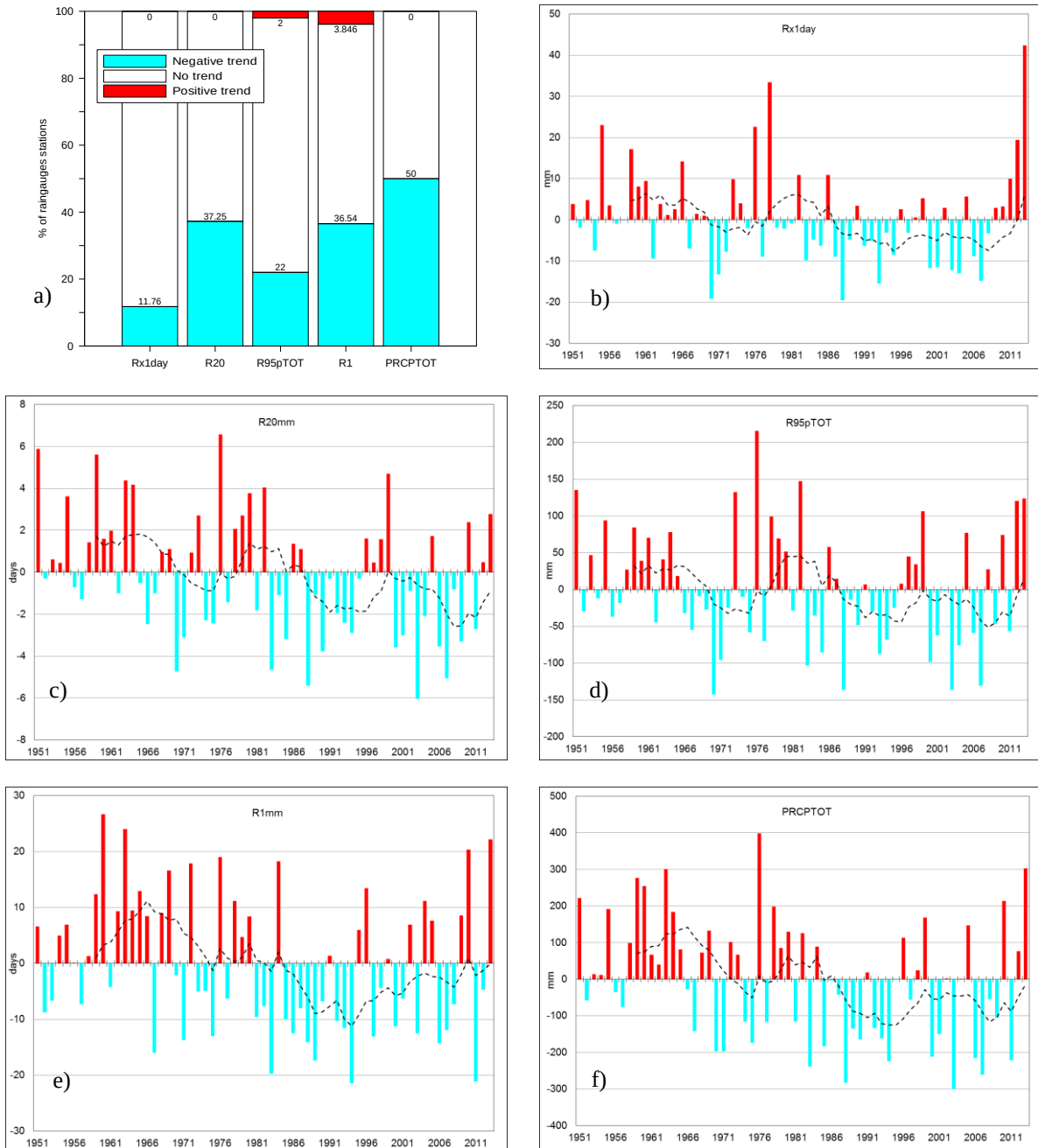
Figure 4. Results of the analysis of ETCCDI indices. (a) Percentage of rain gauges showing a positive, negative and no trend according to the Mann-Kendall test for a significance level \alpha=0.05 ; (b-f) time series of the annual average anomalies of over the period 1951-2013 computed respect to the average value of the climatological normal 1961-1990: (b) Rx1day, (c) R20mm, (d) R95pTOT, (e) R1mm and (f) PRCPTOT. Dashed lines represent the moving average computed over 9 years.
