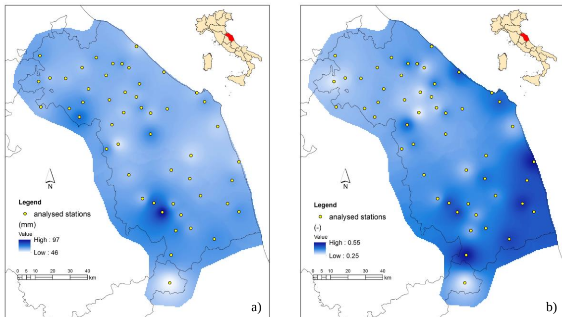
Figure 2. Spatial distribution of the annual maximum daily rainfall in the period 1951-2013 over the region reconstructed by IDW technique. a) mean value; b) coefficient of variation.
